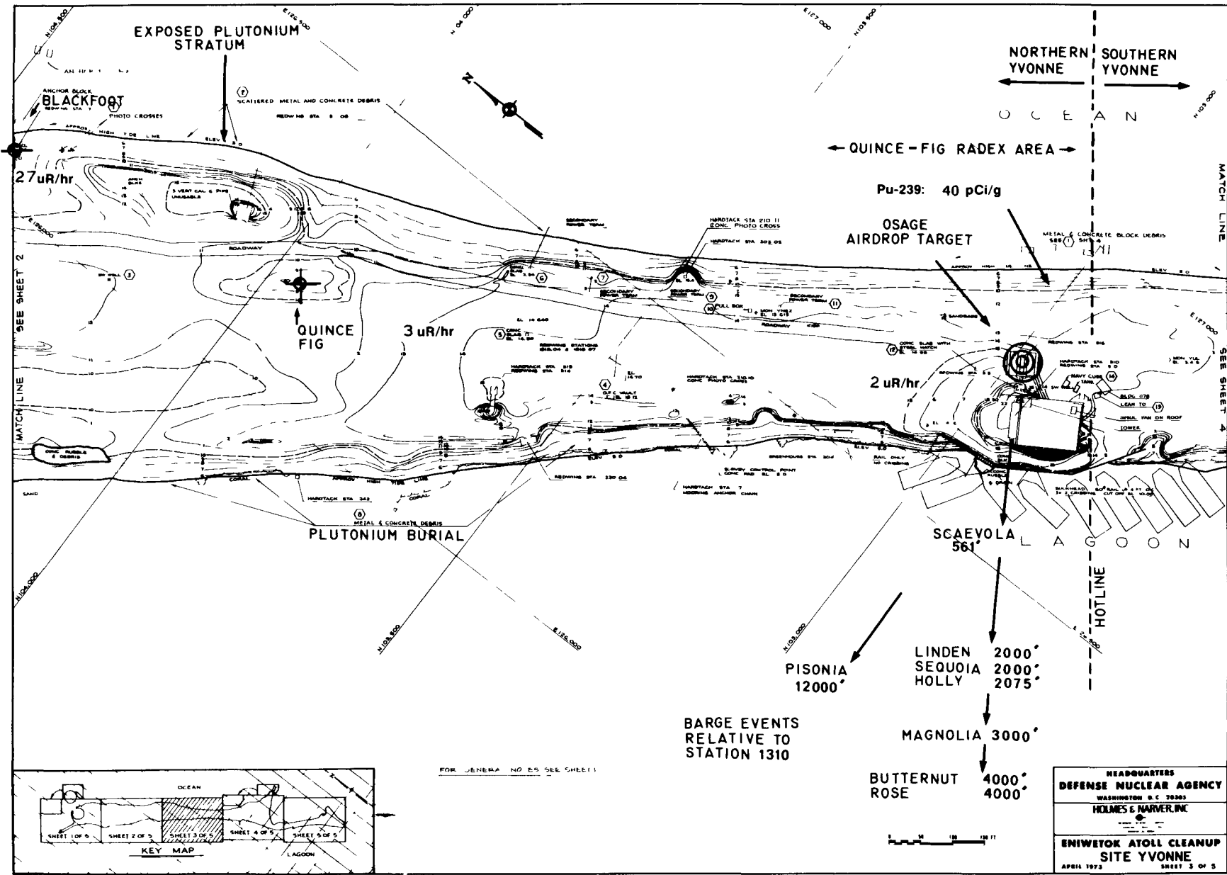
FIGURE 70. SITE YVONNE, SHEET 3 OF 5, NORTH END
